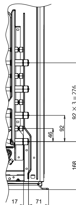
Side view (Valve part)
